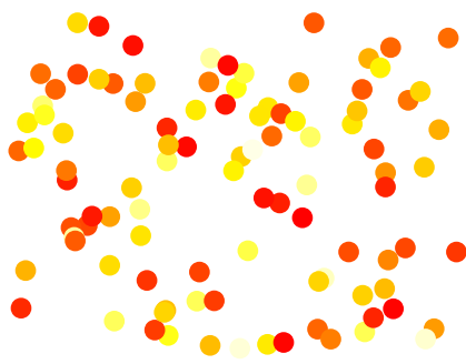
random scatter plot
